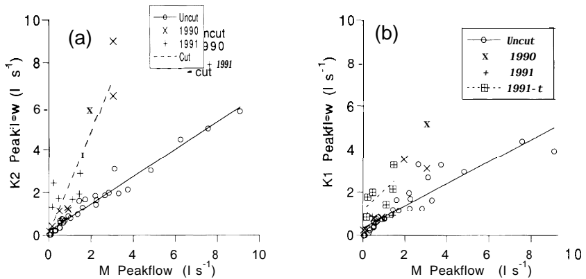
Fig. 2 Relationship between peak pipeflow in uncut control swale M and swales (a) K2 and (b) K1 before and after logging was completed in August 1989. For K1, 1991+ indicates the sum of pipeflow from site K1 and that from a new outlet about 30 m upslope.
